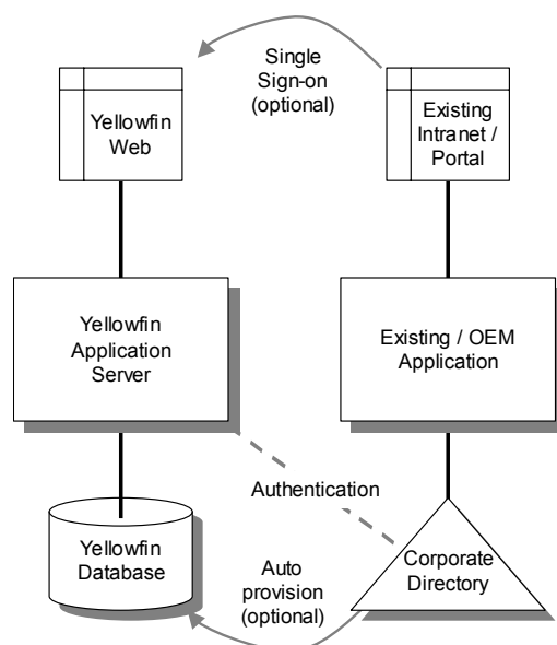
Shared Authentication.
